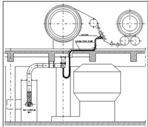
Advanced Knife Dust Removal System Layout
